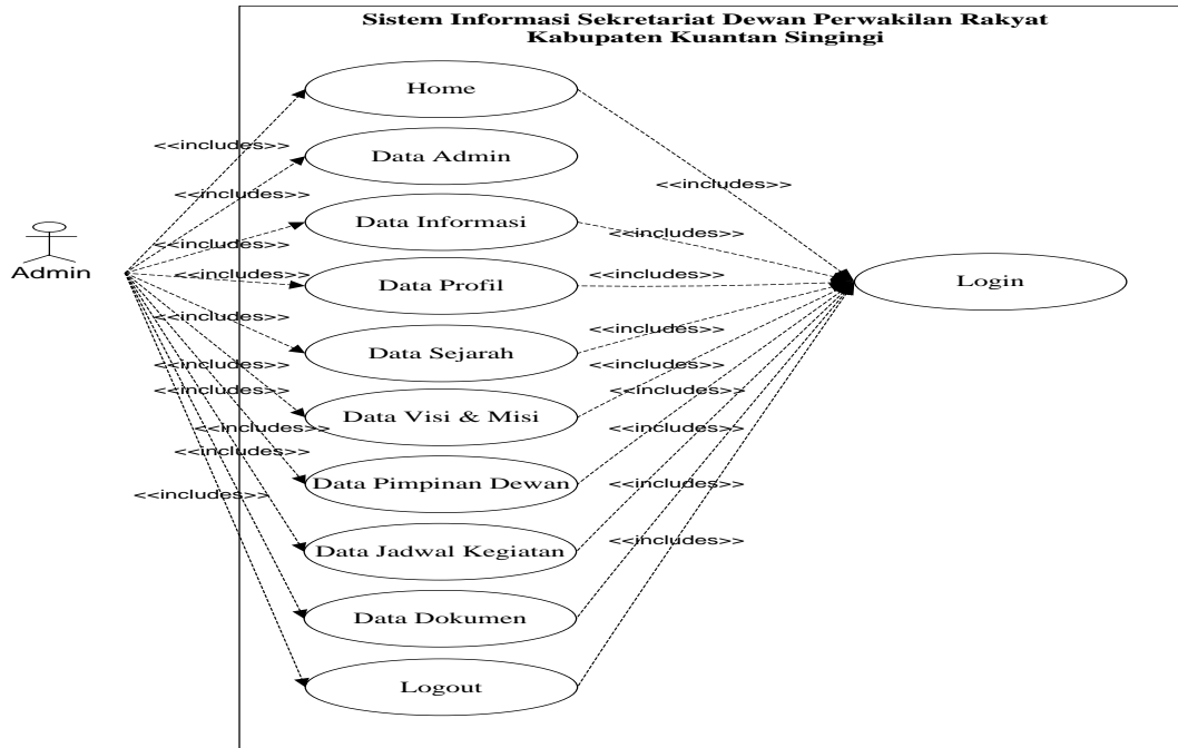
Gambar 4. Use Case Diagram Admin
