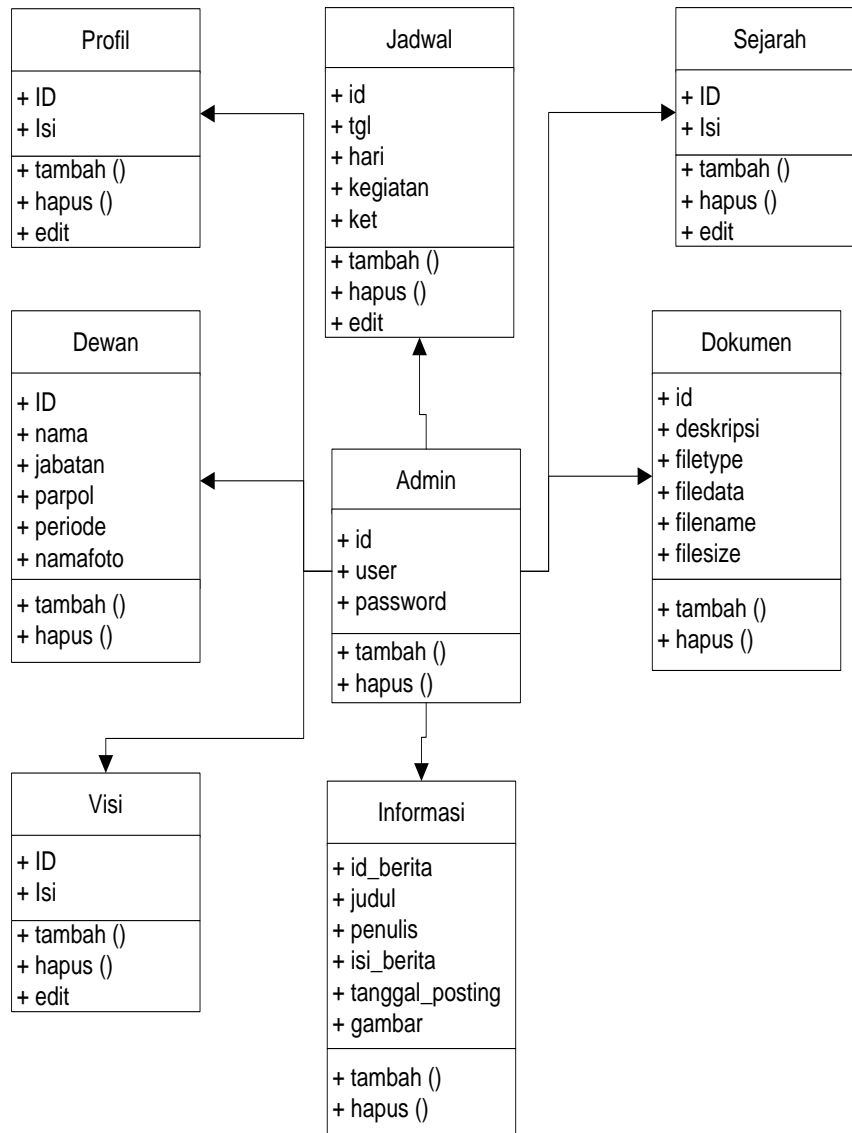
Gambar 6. Class Diagram
