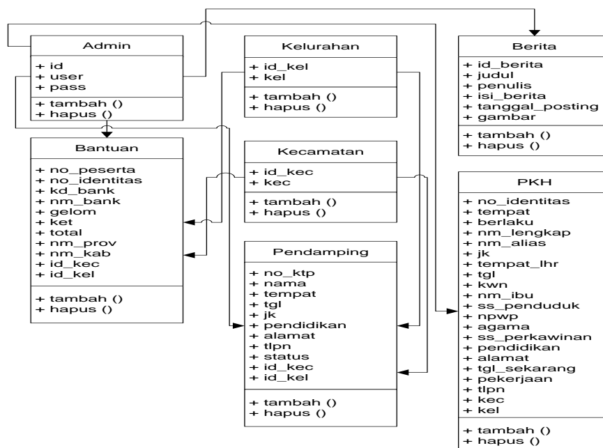
Gambar 5. Class Diagram
