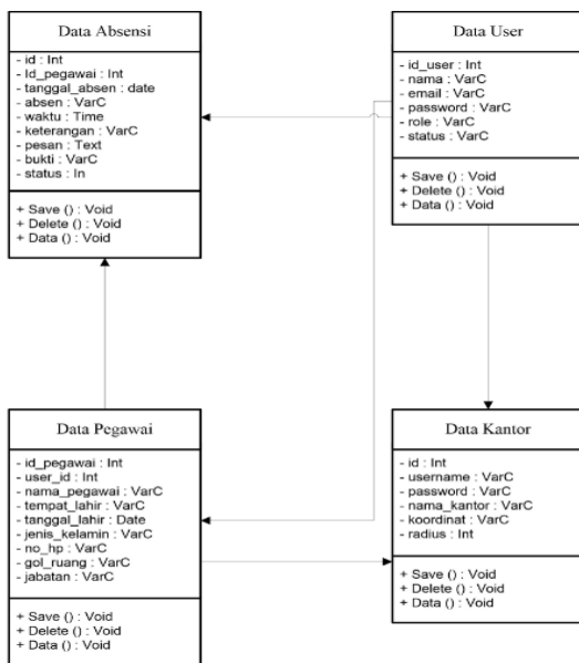
Gambar 3. Class Diagram
