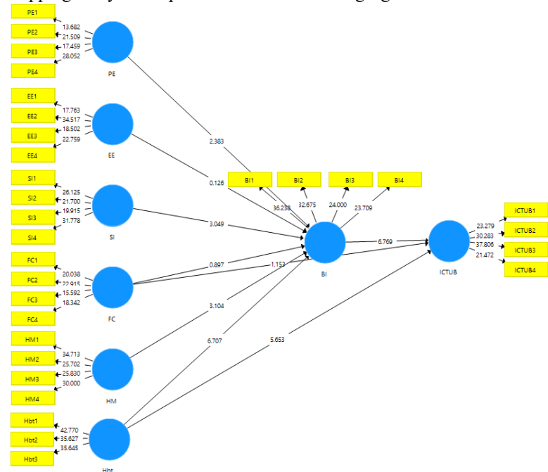
Figure 2. Bootstrapping Results
