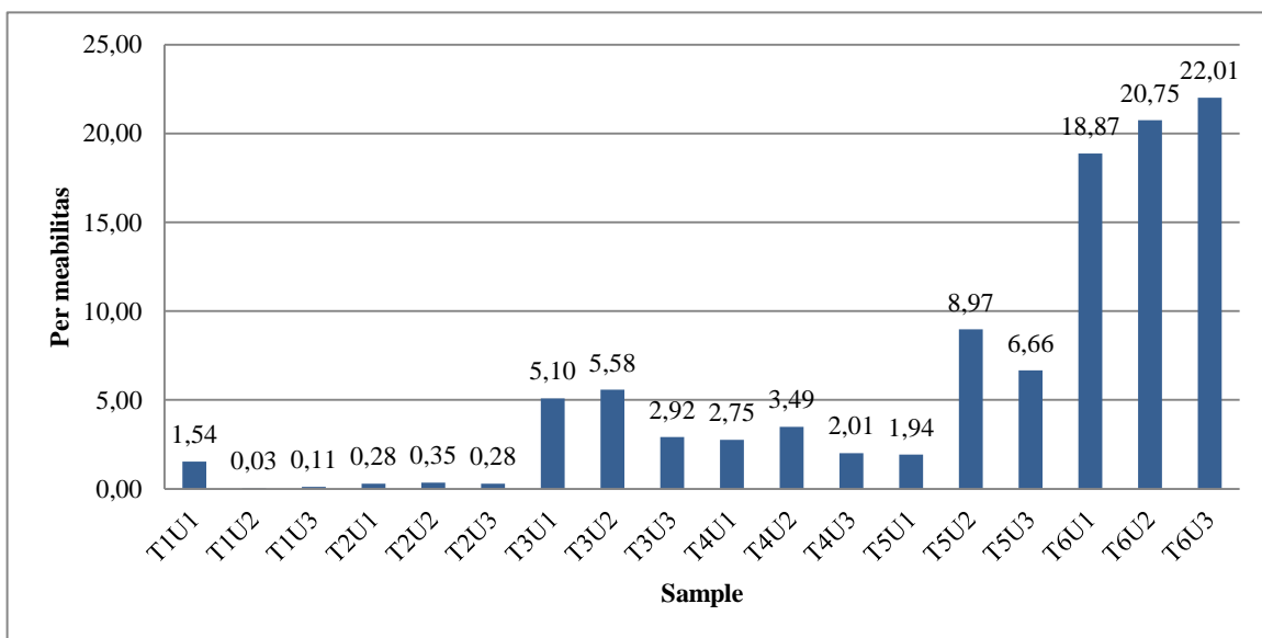
Figure 4. Permeability Results
