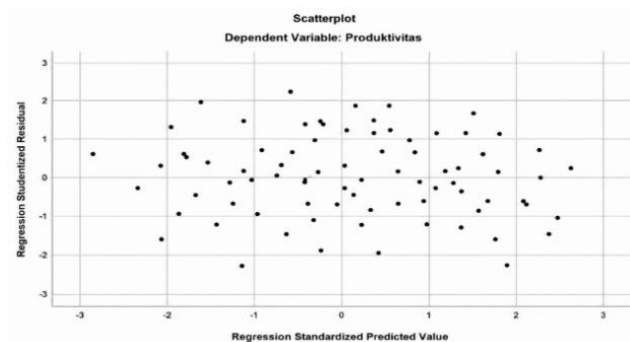
Figure 2. Scatterplot Test Results. Source: Data processed in SPSS 26, 2025
