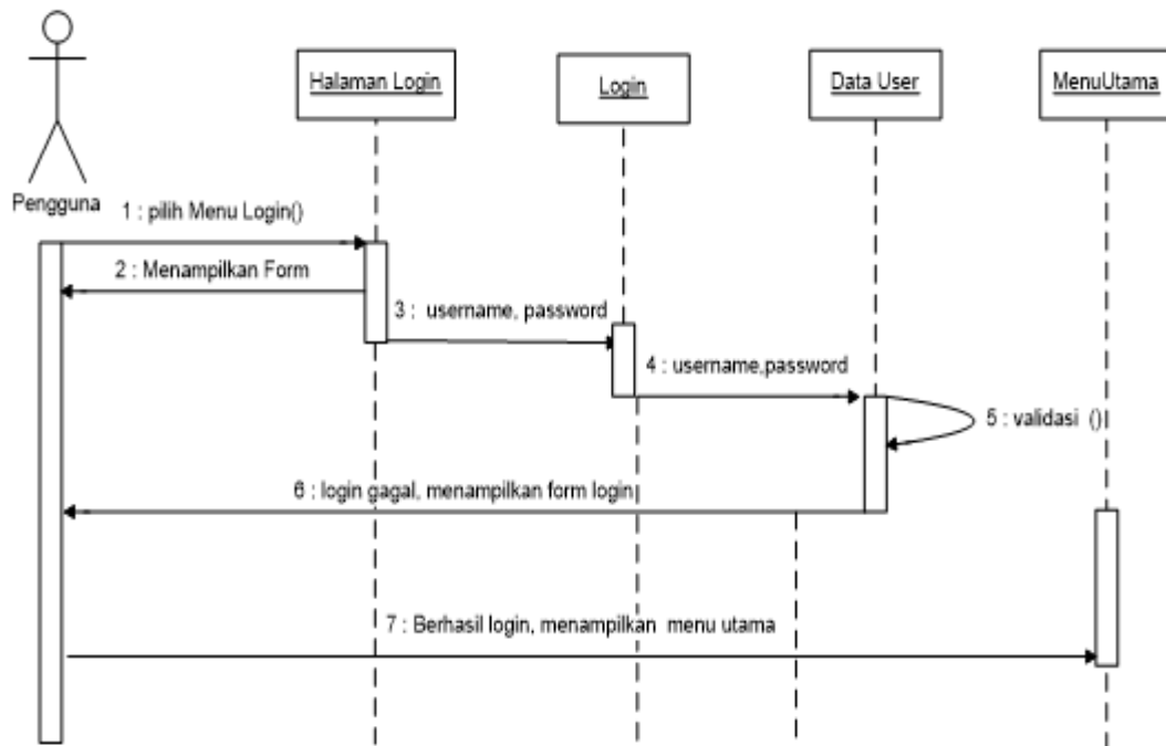
Gambar 4. Sequence Diagram
