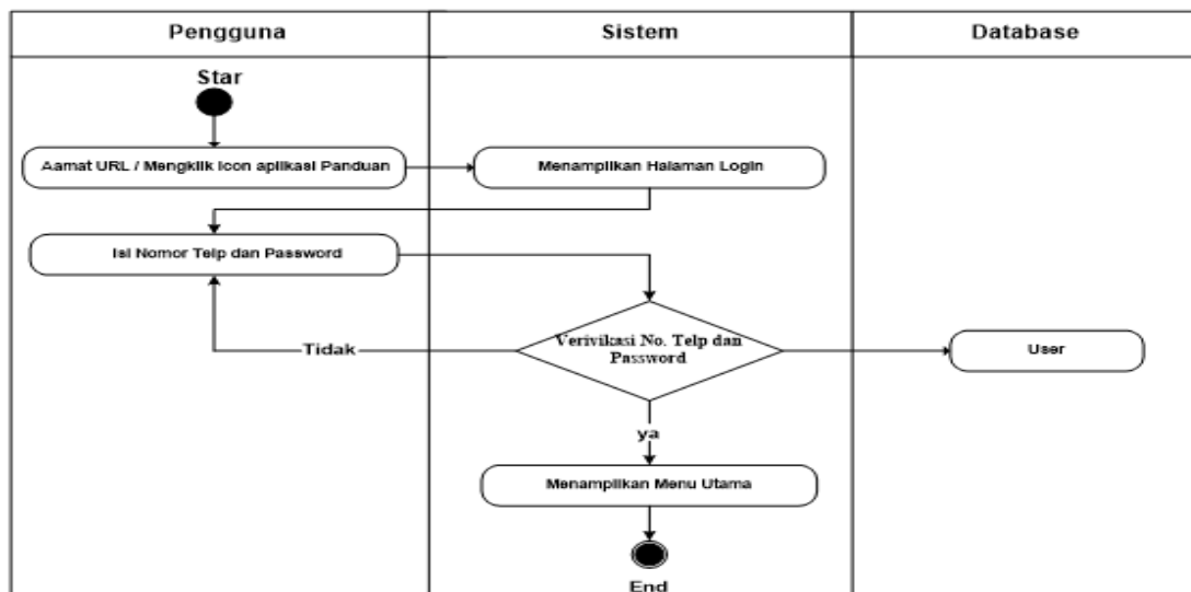
Gambar 3. Activiy Diagram
