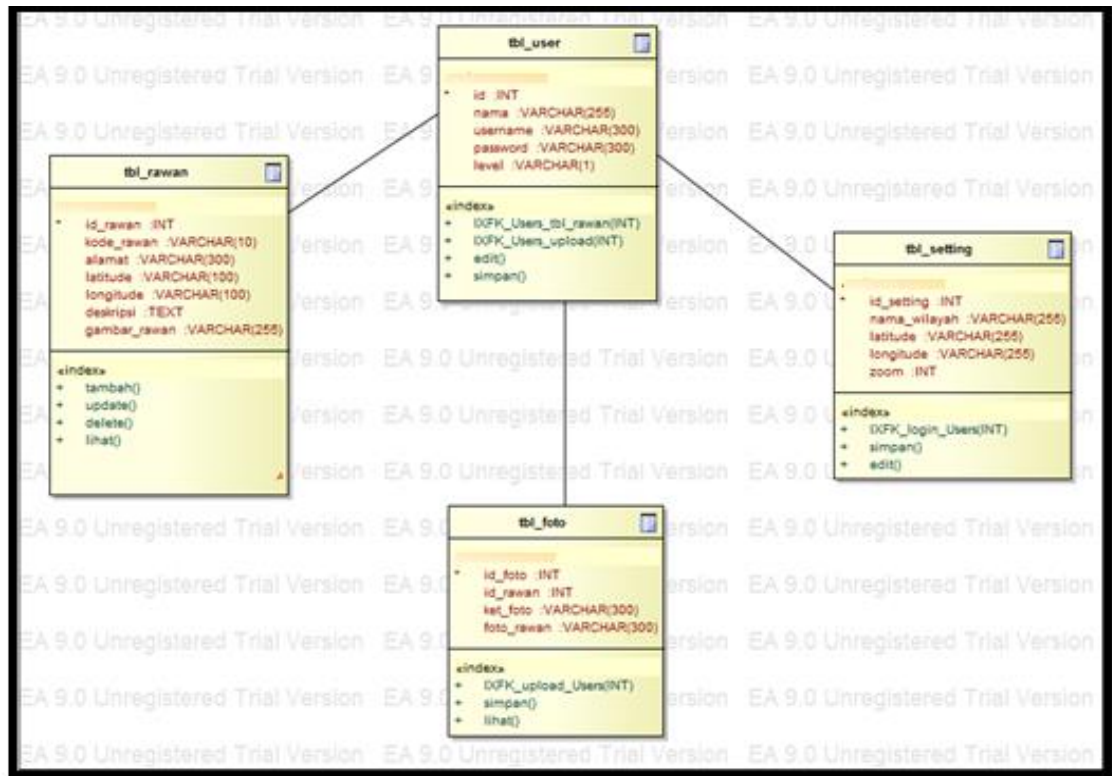
Gambar 3. Class Diagram
