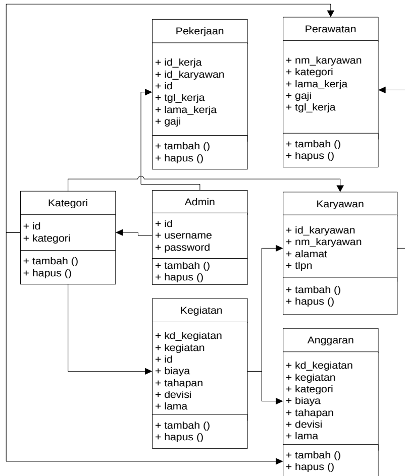
Gambar 4. Class Diagram
