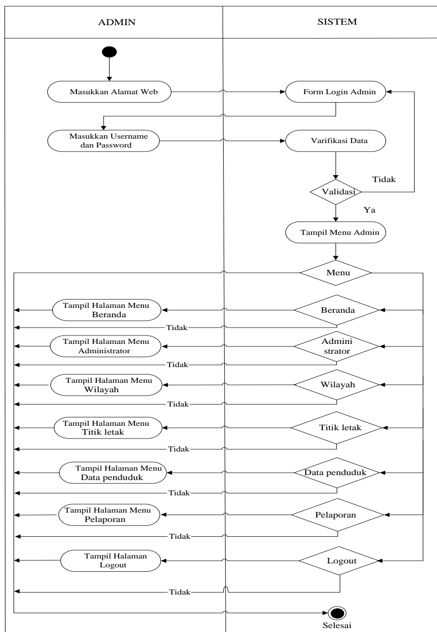
Gambar 4. Activity Diagram Admin
