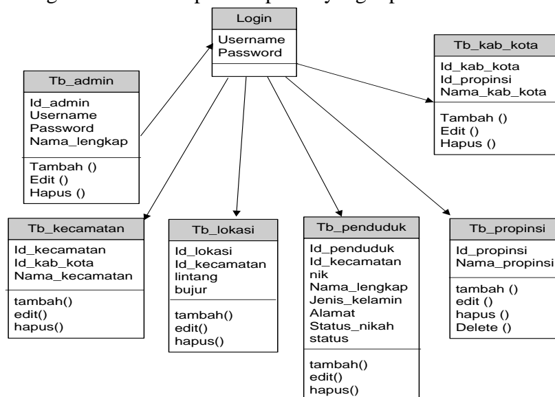
Gambar 6. Class Diagram
