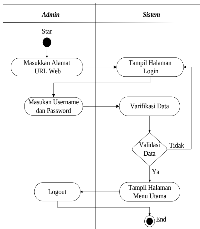
Gambar 4. Activity Diagram
