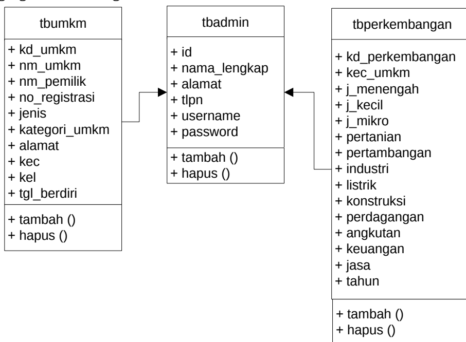
Gambar 6. Class Diagram
