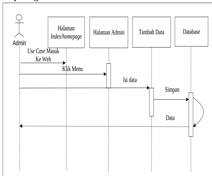
Gambar 5. Squence Diagram
