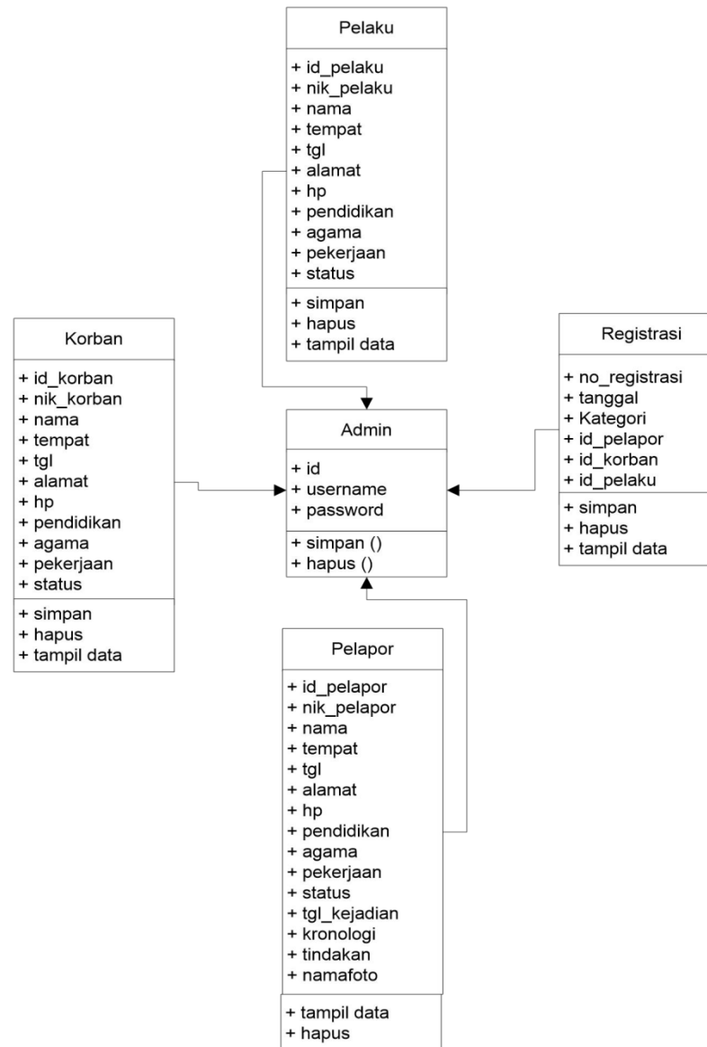
Gambar 5. Class Diagram
