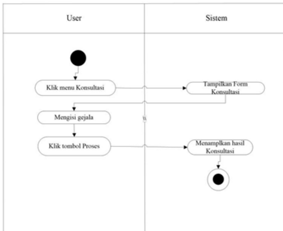
Gambar 3. Activity Diagram Konsultasi
