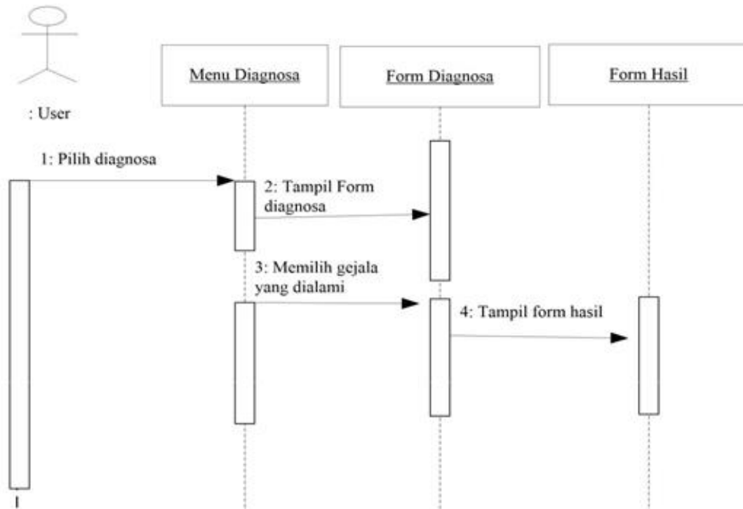
Gambar 4. Sequence Diagram Diagnosa
