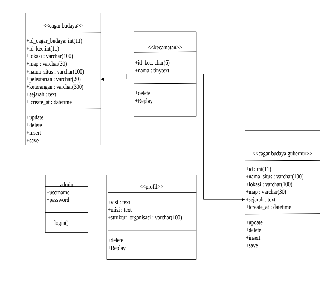
Gambar 2. Class Diagram
