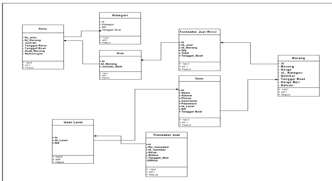
Gambar 5. Class Diagram
