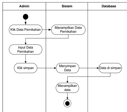
Gambar 3. Activity Diagram Admin Mengelola Data Pernikahan
