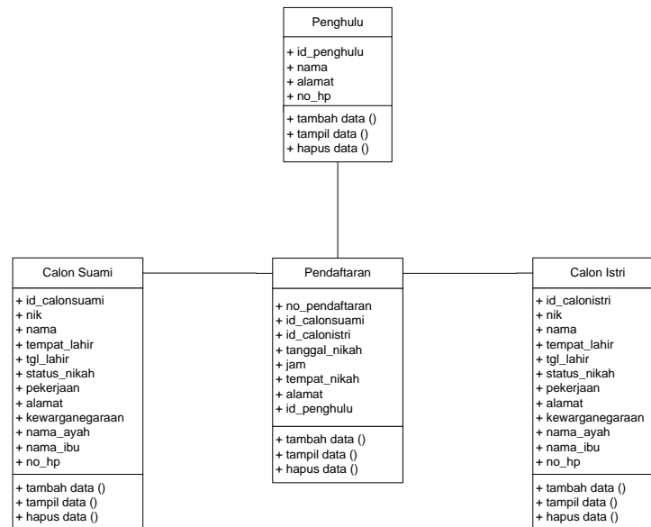
Gambar 11. Class Diagram
