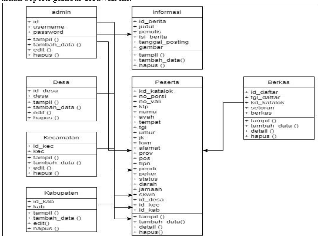
Gambar 7. Class Diagram
