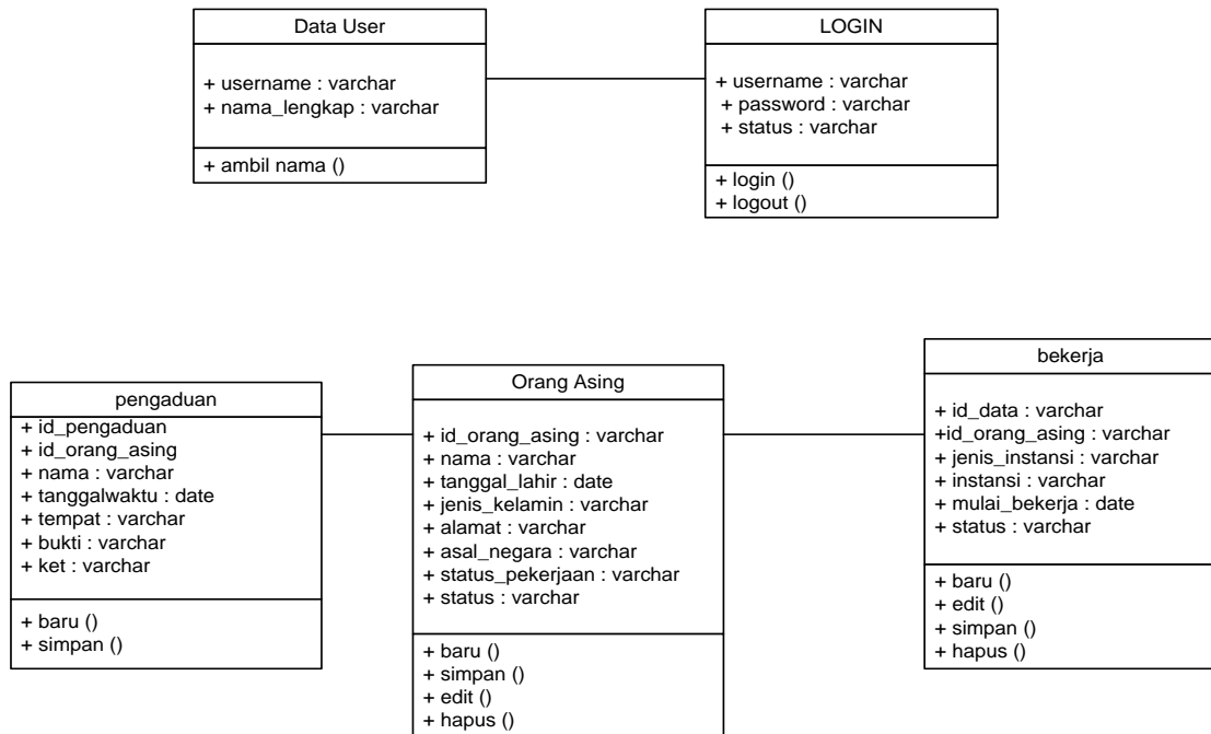
Gambar 5. Class Diagram
