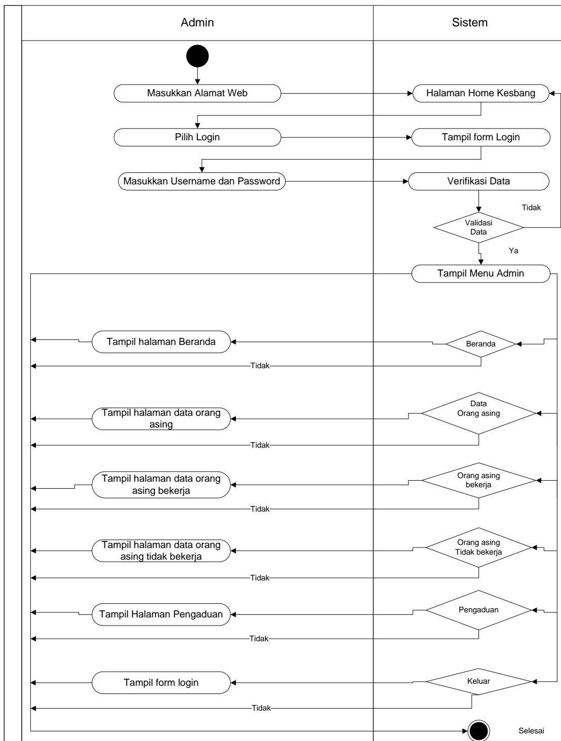
Gambar 4. Activity Diagram Admin
