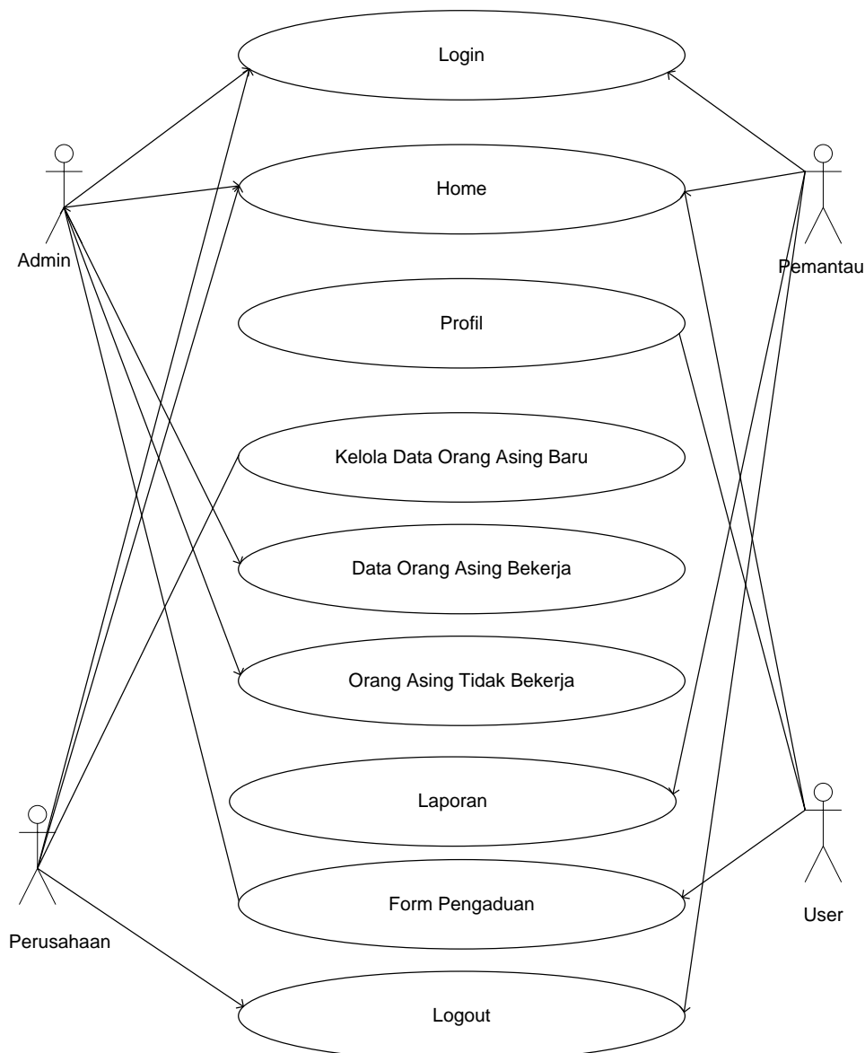
Gambar 3. Use Case Diagram
