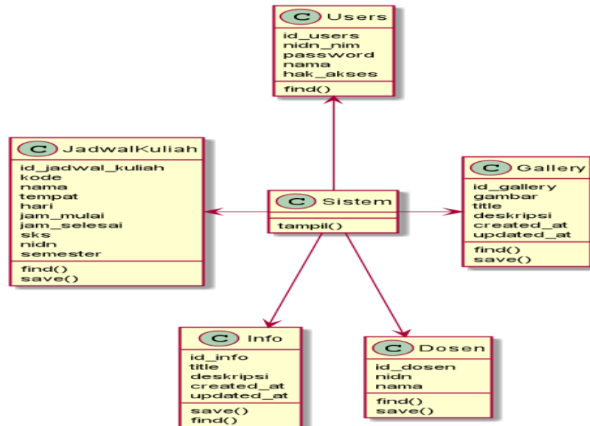
Gambar 3. Class Diagram
