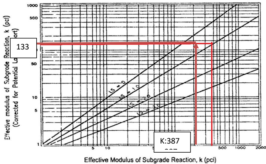
Gambar 4. Correction of Effective modulus of Subgrade Reaction for Potential Loss Subbase Support.
