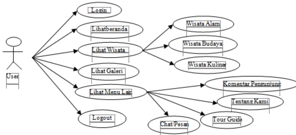
Gambar 6. Use Case Diagram User
