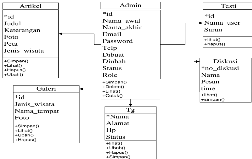
Gambar 7. Class Diagram
